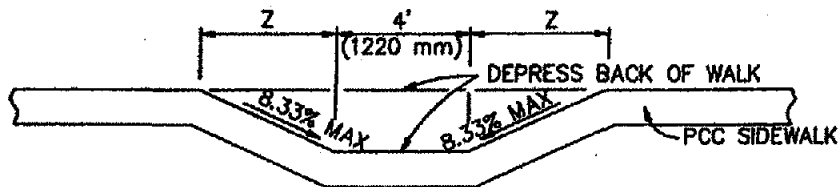
SECTION R-R
