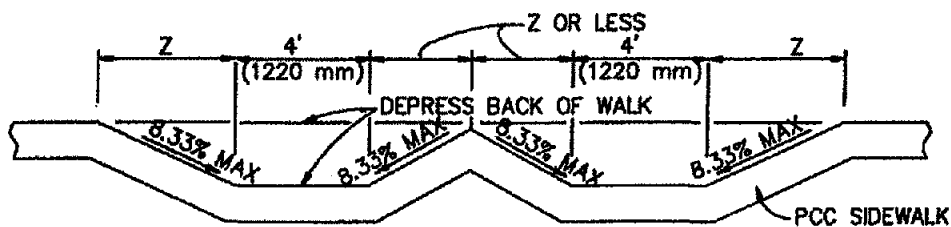
SECTION S-S
